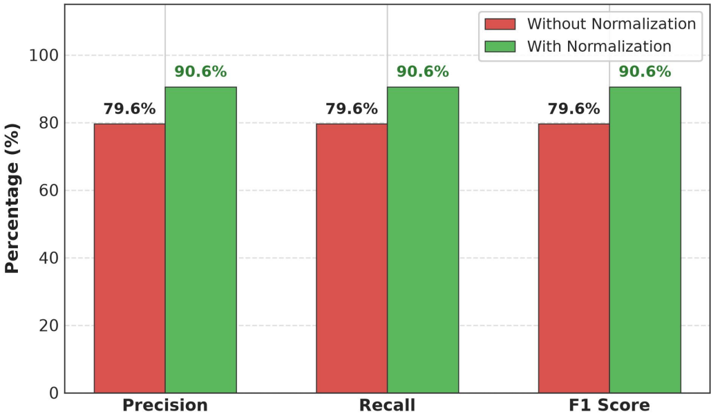
Fig. 4. Accuracy Improvement after Semantic Canonical Normalization.
