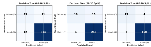
Fig. 8. Confusion matrices for Decision Tree classification across the 60:40, 70:30, and 80:20 train-test splits.
