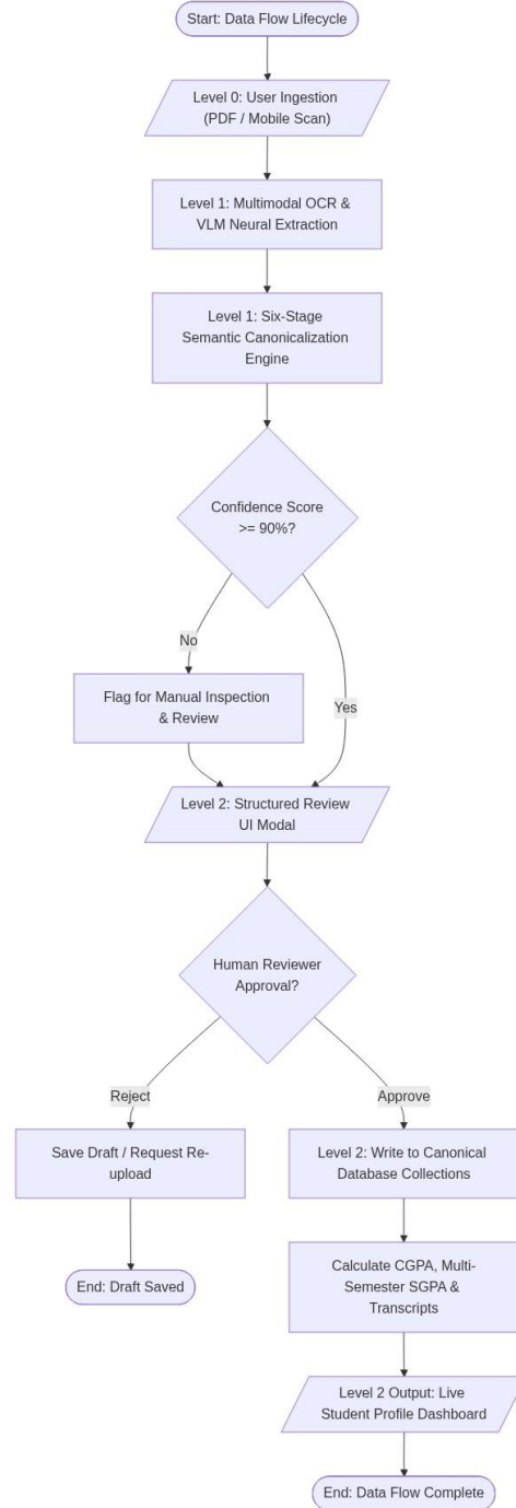
Fig. 2. Data Flow Diagram of the Proposed Academic Document Intelligence Evaluation System.
