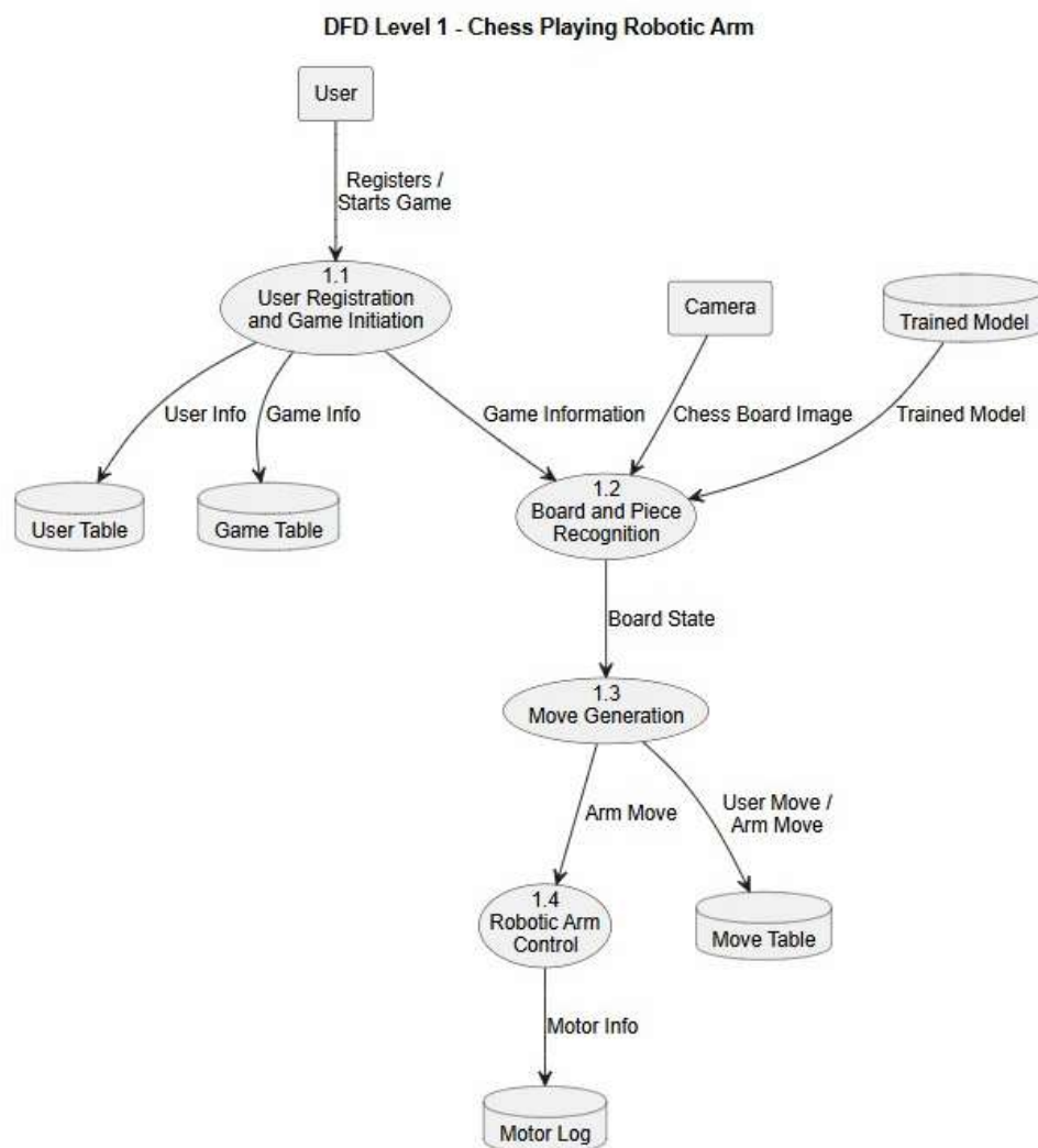
Figure 1.5 Data Flow Diagram
