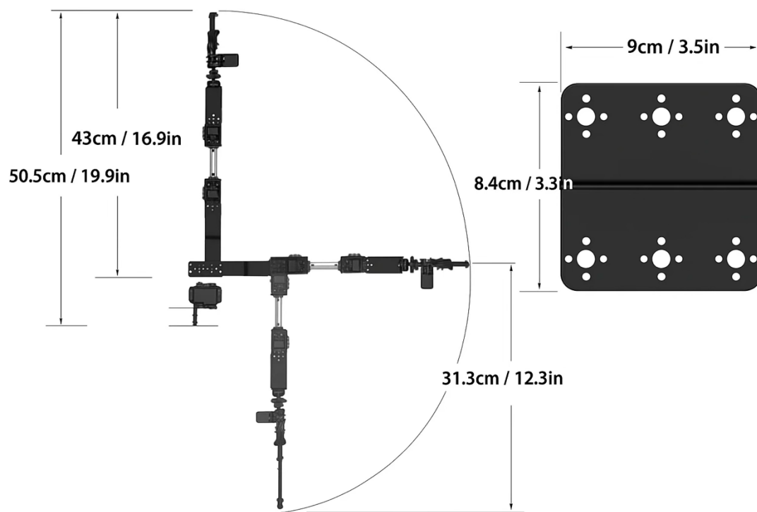
Figure 8.3 Arm reach
