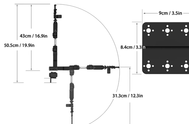
Figure 8.3 Arm reach
