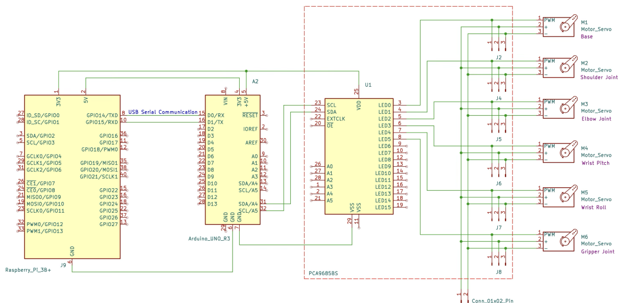
Figure 1.3 Hardware Circuit Diagram
