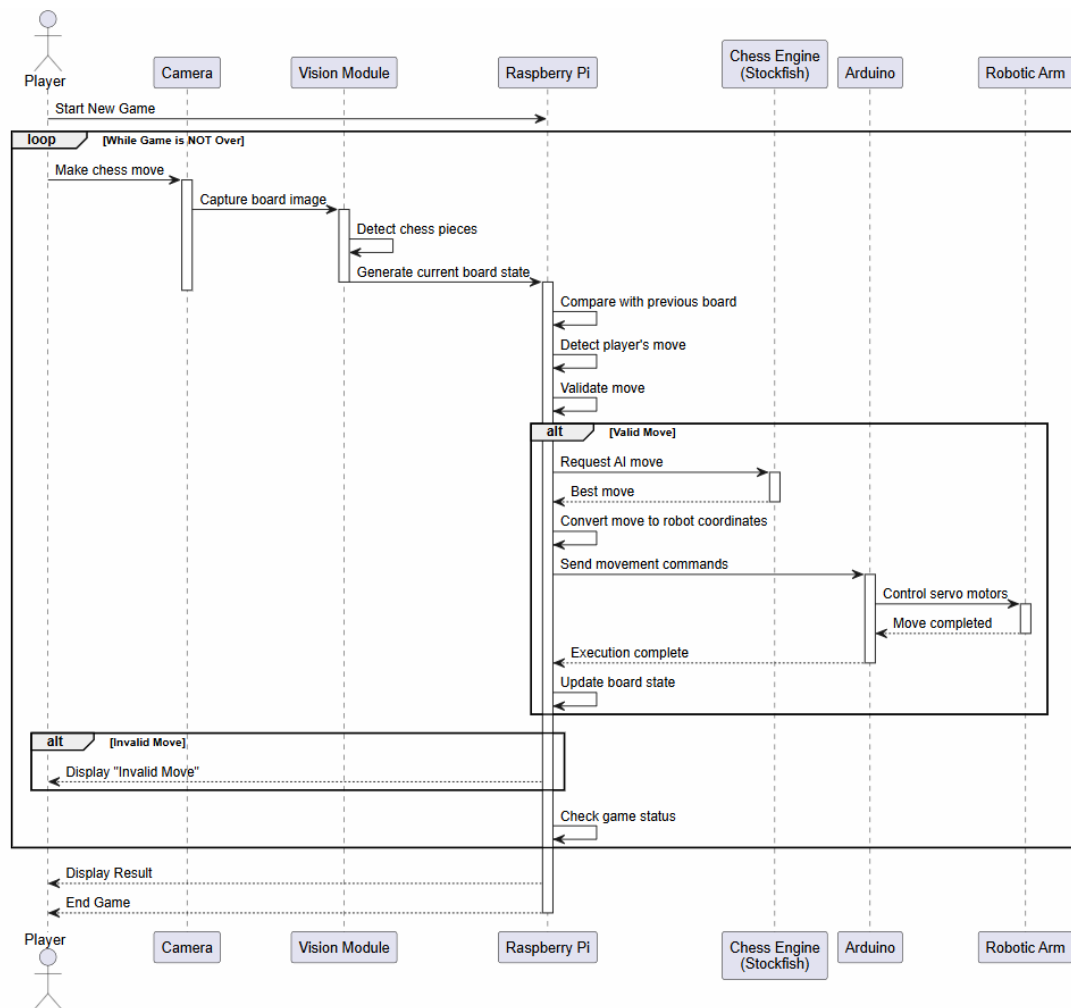
Figure 1.2 Sequence Diagram
