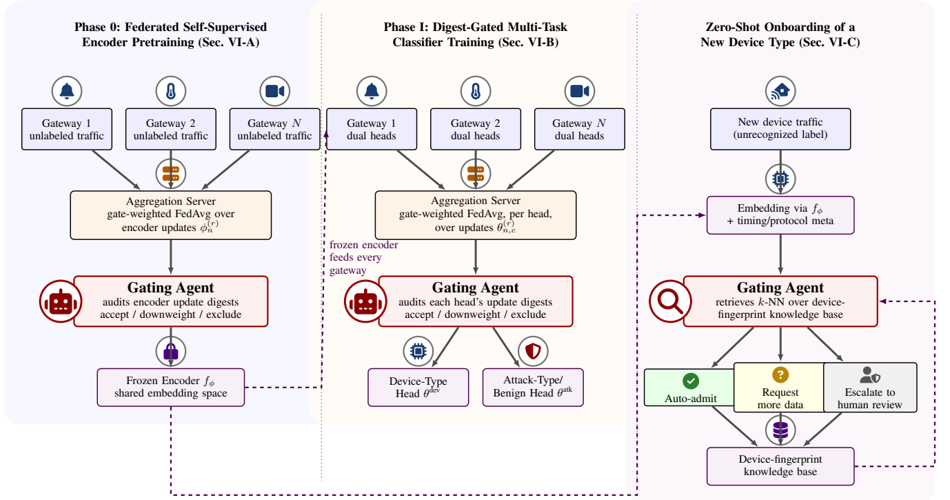
Fig. 1. System overview. The Gating Agent inspects each client’s per-round digest before aggregation (center), a design validated across the federated encoder/classifier training loop and, using the same retrieval signal, at zero-shot device onboarding (right).
