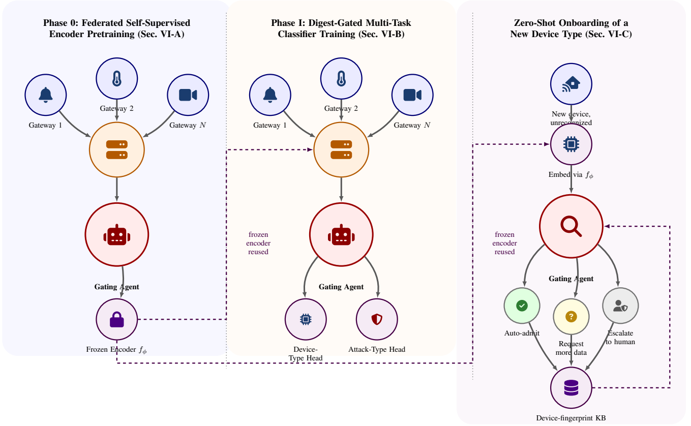
Fig. 1. System overview. The Gating Agent inspects each client’s per-round digest before aggregation (center), a design validated across the federated encoder/classifier training loop and, using the same retrieval signal, at zero-shot device onboarding (right).
