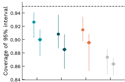
Coverage of realised-normal values
