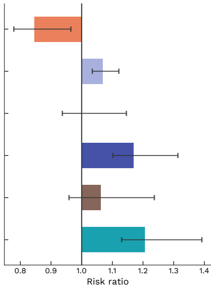
INSPIRE
