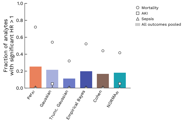
eICU-CRD: within Pop RI -normal tests
