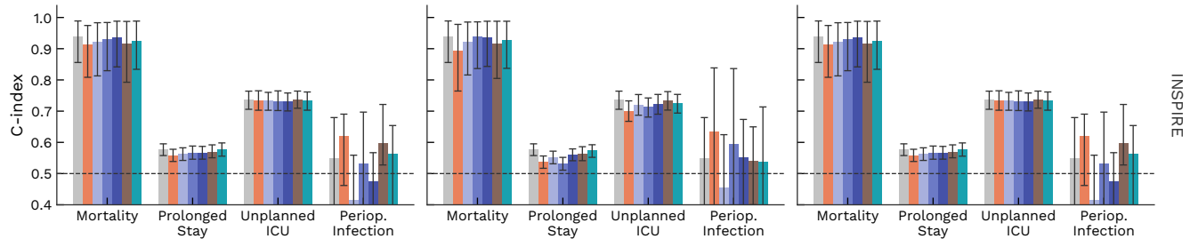
Cox refit per method
