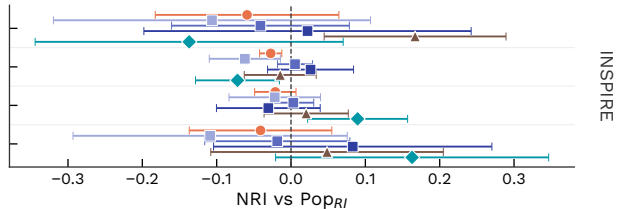
\text{Pop}_{RI} -trained Cox, flags swapped
