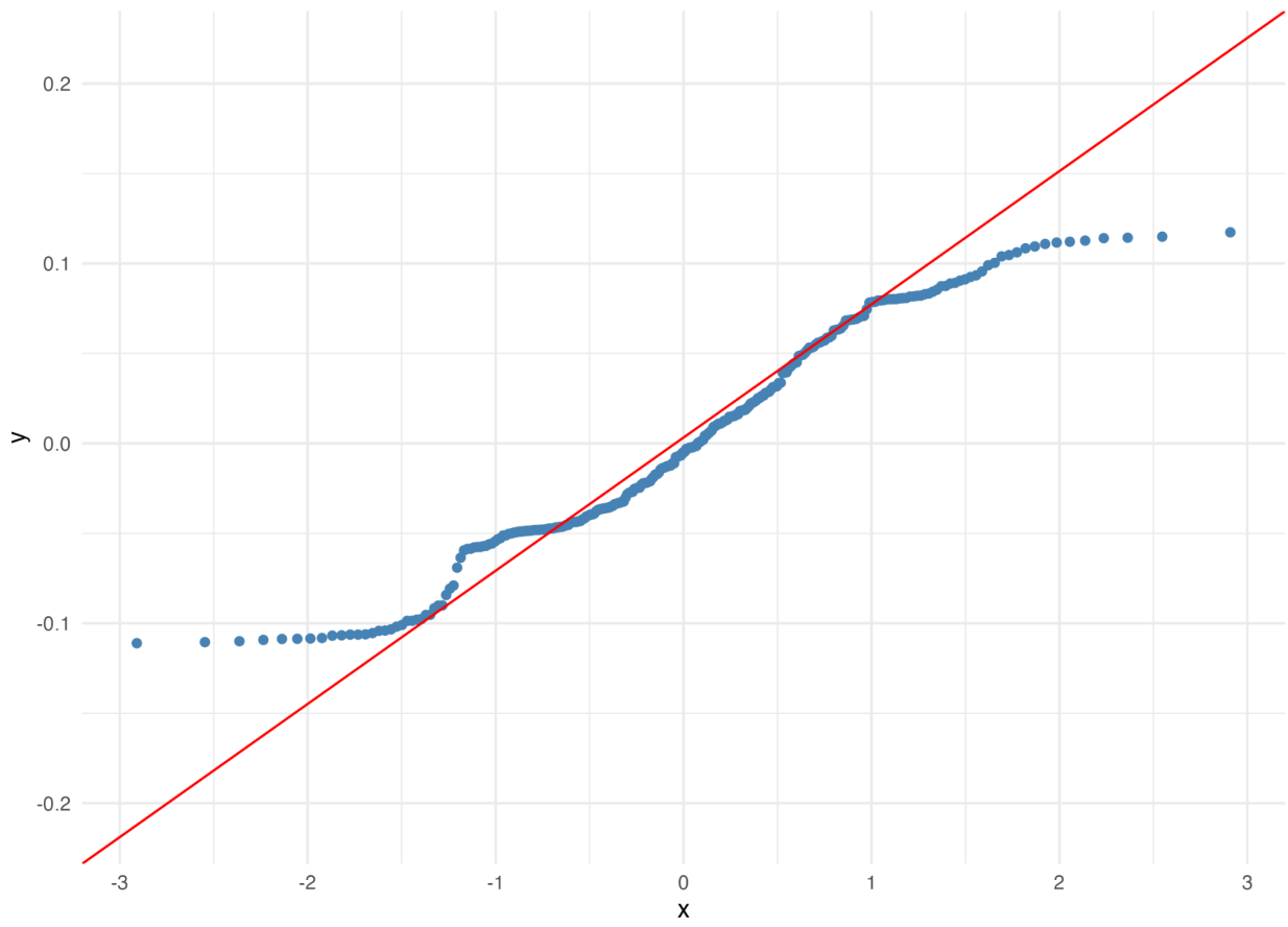
Model Diagnostic: Normal Q-Q Plot of Residuals
