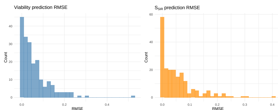
Fig. 6 Prediction accuracy under missingness on DrugCombDB ( n = 200 matrices, 20% interior wells held out). Left: holdout RMSE for viability predictions. Right: holdout RMSE for the SIR synergy summary S_{SIR} . Median prediction error is 0.040 in viability units and 0.035 for S_{SIR} , indicating that the monotone surface captures the underlying dose-response relationship well enough to impute missing measurements. This capability is unique to SIR: existing synergy scores are computed pointwise and cannot predict unobserved dose pairs.
