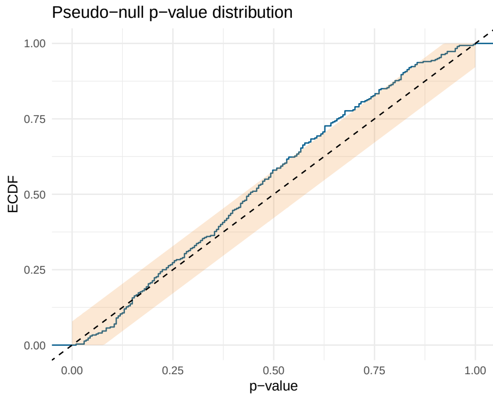
Fig. 3 Pseudo-null calibration on DrugCombDB ( n = 300 randomly selected matrices; B = 200 ). P-values from the df-corrected wild bootstrap when data are generated under the fitted additive null by sign-flipping corrected residuals, so that no true interaction is present by construction. The dashed diagonal is the Uniform(0, 1) reference expected for a well-calibrated test; the shaded region is a 95% Dvoretzky-Kiefer-Wolfowitz band. The close agreement with the uniform diagonal demonstrates that SIR's p-values are trustworthy on real screening data with real noise structure, not just in controlled simulations (Fig. 4).
