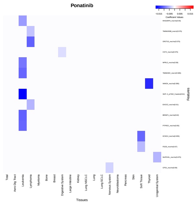
Fig. 19. Heatmap of mean coefficient estimates from 200 bootstrap replicates of the DSEN model for Ponatinib. The proportion of times the shared or tissue-specific coefficient estimates were non-zero in the bootstrap replicate is indicated in parenthesis beside the corresponding feature name. The 15 features with the highest non-zero proportion are presented. SHP-2 expression has the largest negative mean coefficient estimate, indicating it is an important predictor for cell line sensitivity to Ponatinib. SHP-2 is necessary for leukemogenesis and is in the targeted pathway of Ponatinib [9].
