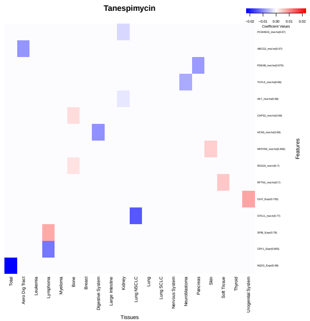
Fig. 18. Heatmap of mean coefficient estimates from 200 bootstrap replicates of the DSEN model for Tanespimycin. The proportion of times the shared or tissue-specific coefficient estimates were non-zero in the bootstrap replicate is indicated in parenthesis beside the corresponding feature name. The 15 features with the highest non-zero proportion are presented. In our model, NQO1 expression is associated with increased sensitivity to Tanespimycin treatment in all tissue types.
