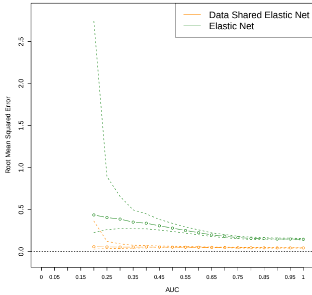
Fig. 16. Comparison of RMSE between the DSEN and EN models for Tanespimycin in cell lines with an observed AUC value less than or equal to a specified threshold. The dashed lines represent the 95% confidence intervals. The DSEN model demonstrates a lower RMSE than the EN model for cell lines exhibiting higher sensitivity to Tanespimycin treatment.
