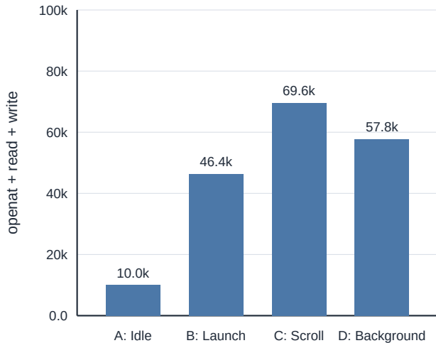
File syscall intensity
