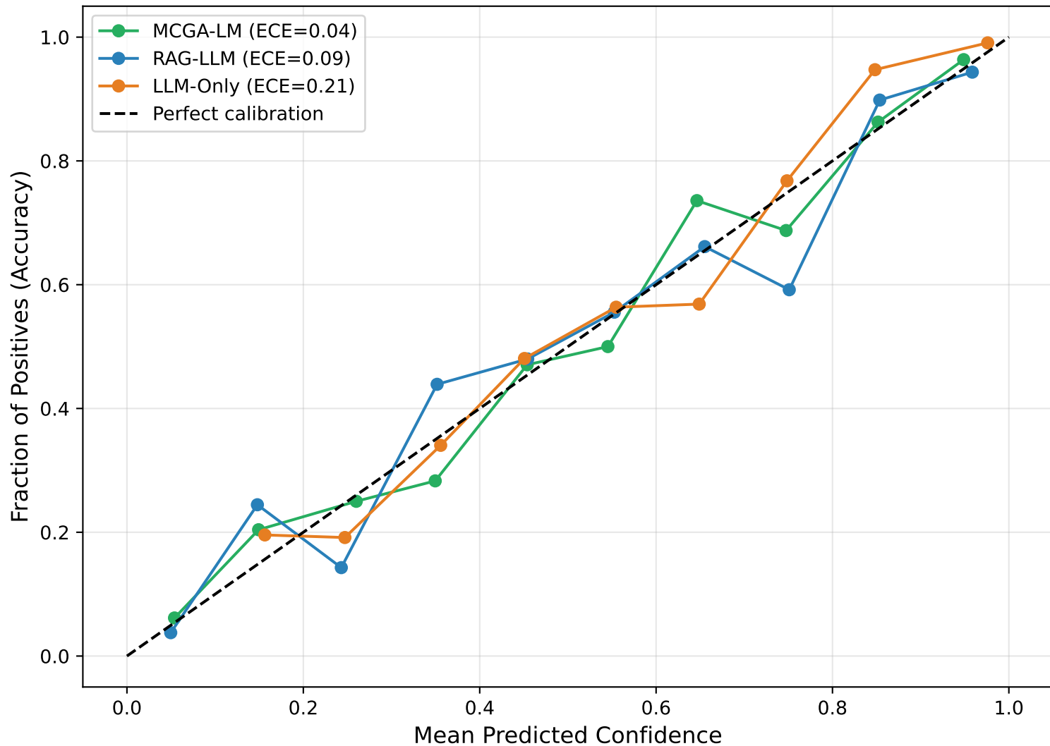
Confidence Calibration Curves
