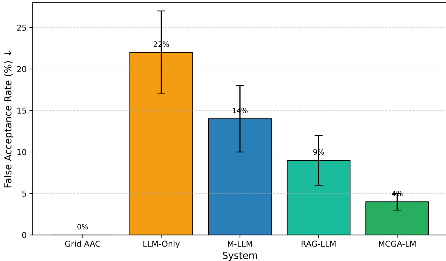
Safety: Utterances Accepted but Incorrect (Lower is Better)
