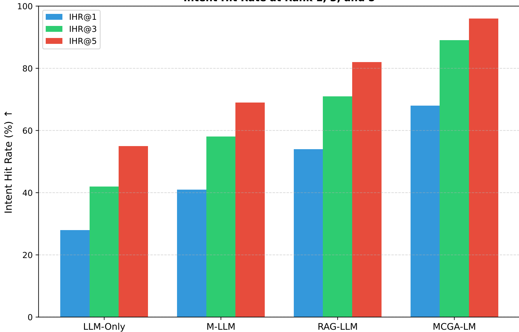
Intent Hit Rate at Rank 1, 3, and 5
