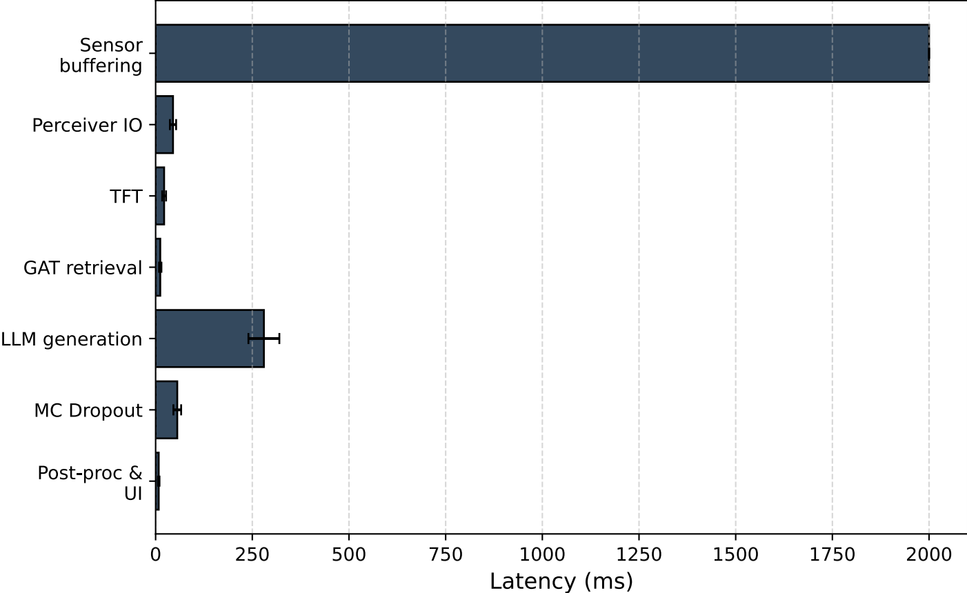
End-to-End Inference Latency Breakdown
