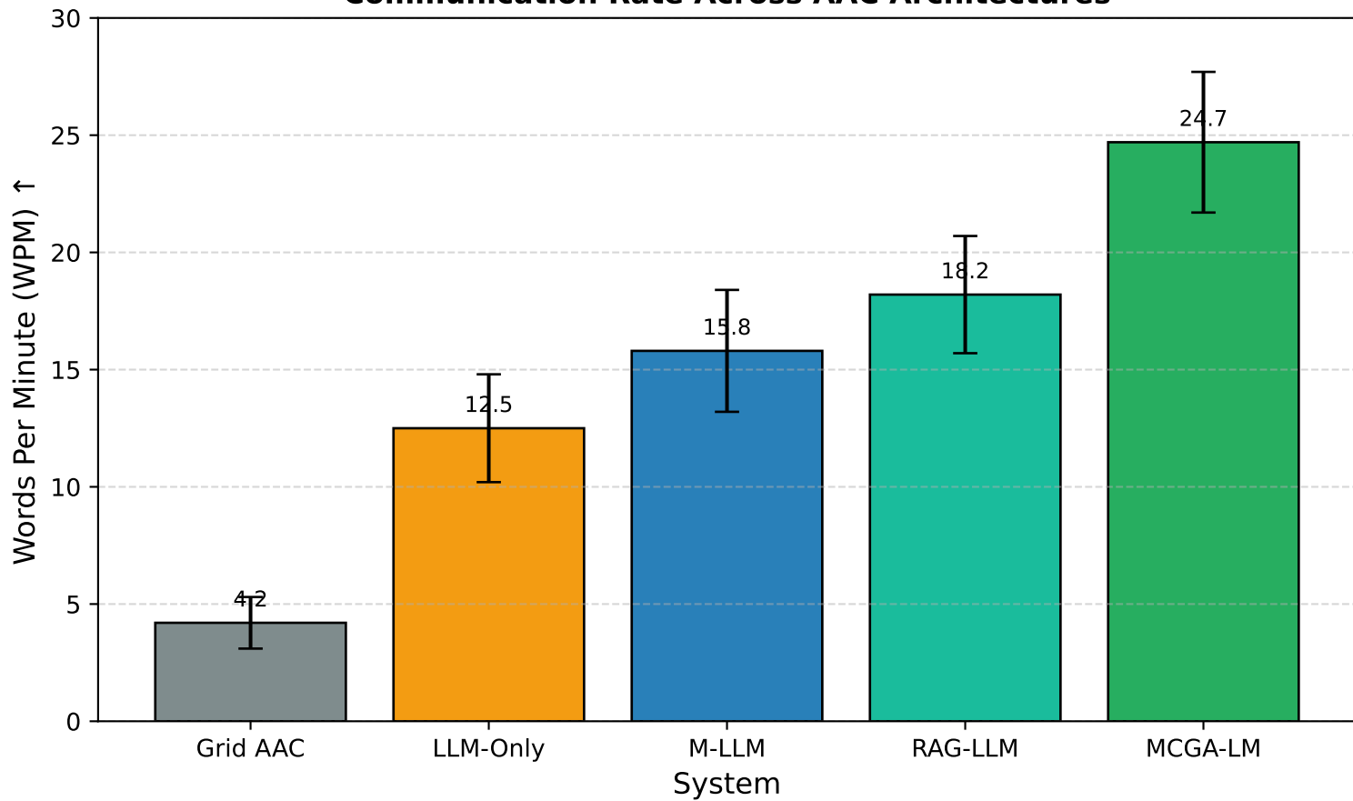
Communication Rate Across AAC Architectures
