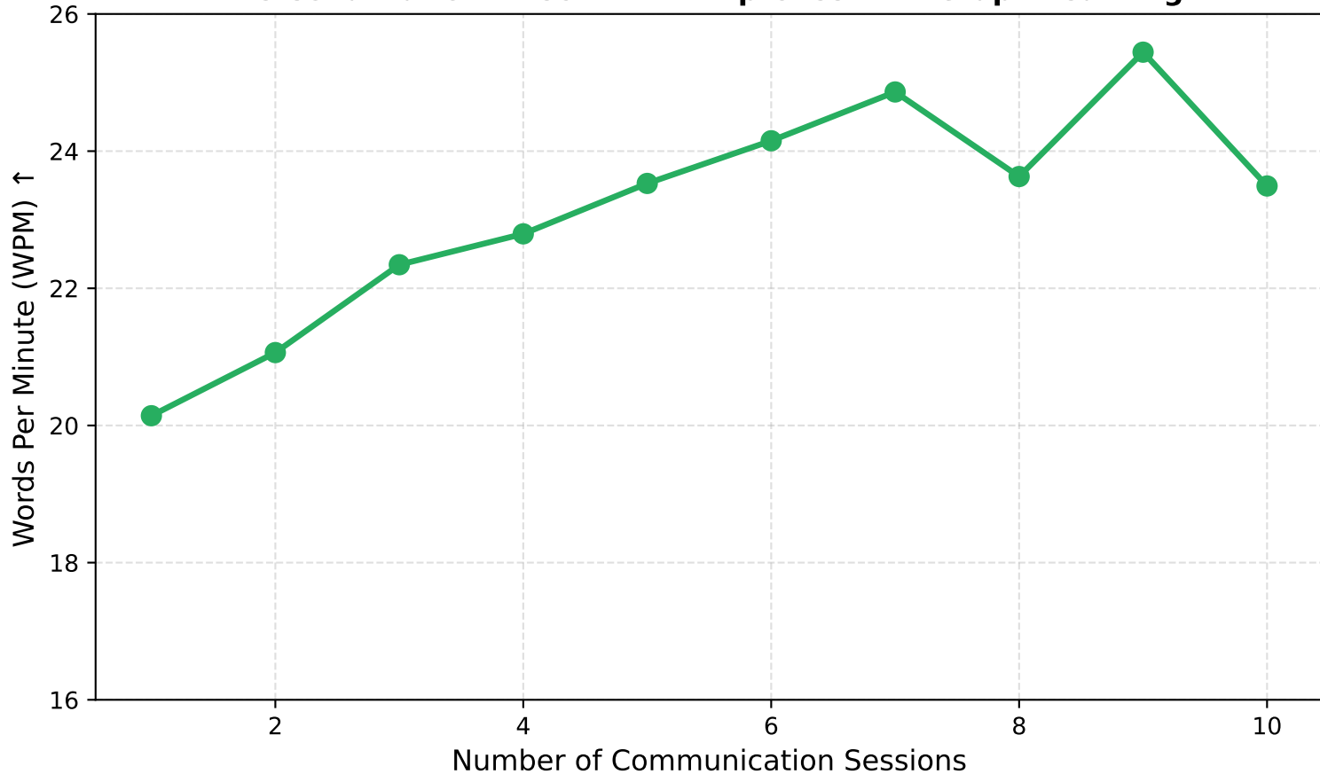
Personalization Effect: WPM Improves with Graph Learning
