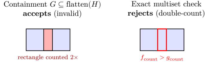
Figure 3: Why exact rectangle-multiset certification matters. Greedy growth over a dense periodic region can place two cell instances that overlap, reproducing a rectangle twice. A containment check ( G \subseteq \text{flatten}(H) ) accepts this invalid tiling; the exact multiset check requires every real rectangle to appear with exactly its multiplicity and rejects the double-count. This is the check that caught the over-covering bug.
