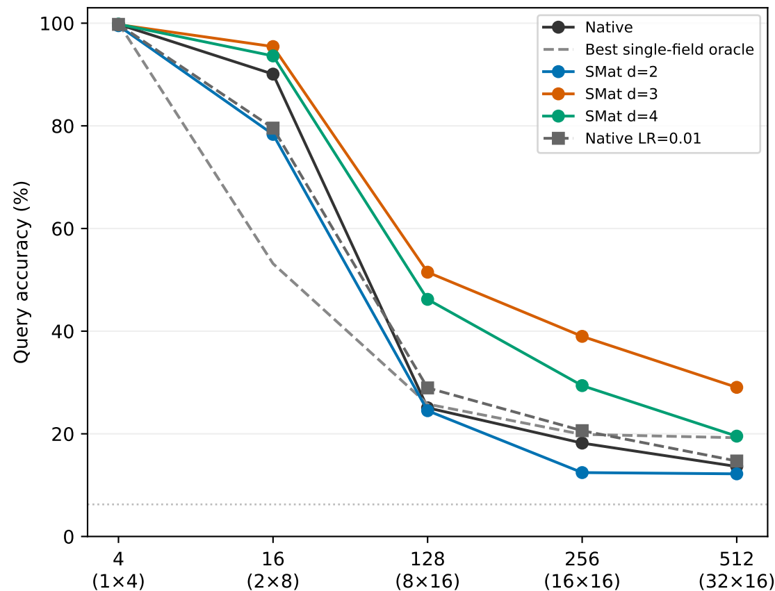
Gated DeltaNet
