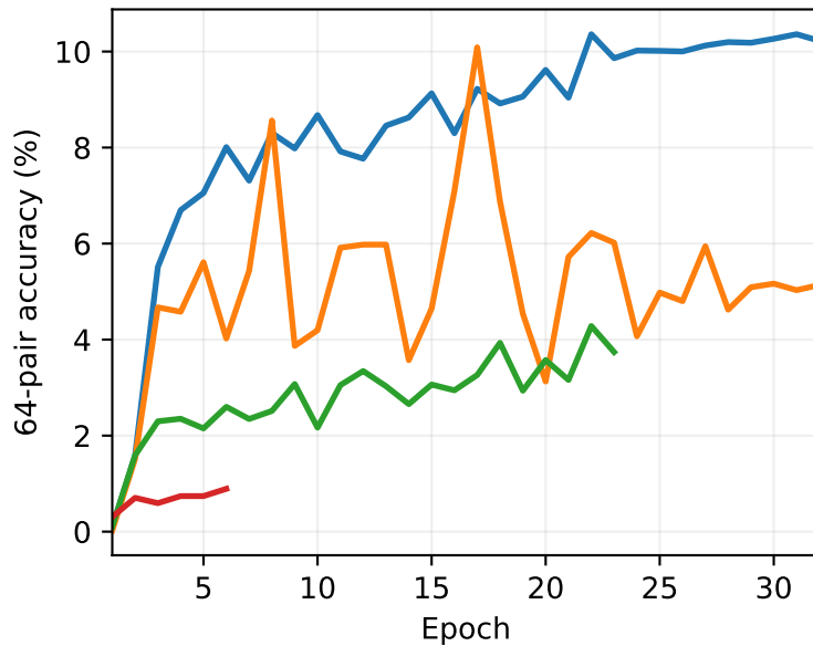
MQAR: width 32, 2 heads, head/state 16; seed 123, LR 0.01
