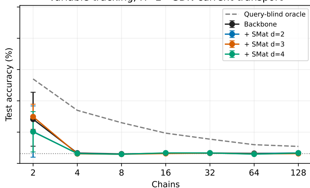
Variable tracking, H=2 · GDN current transport
