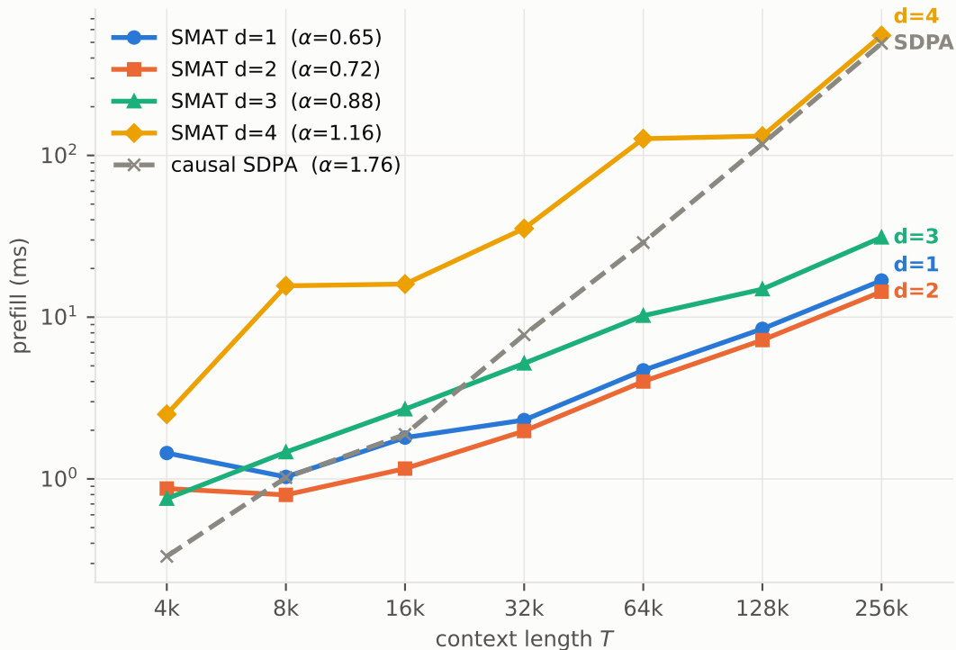
Prefill cost against causal attention
