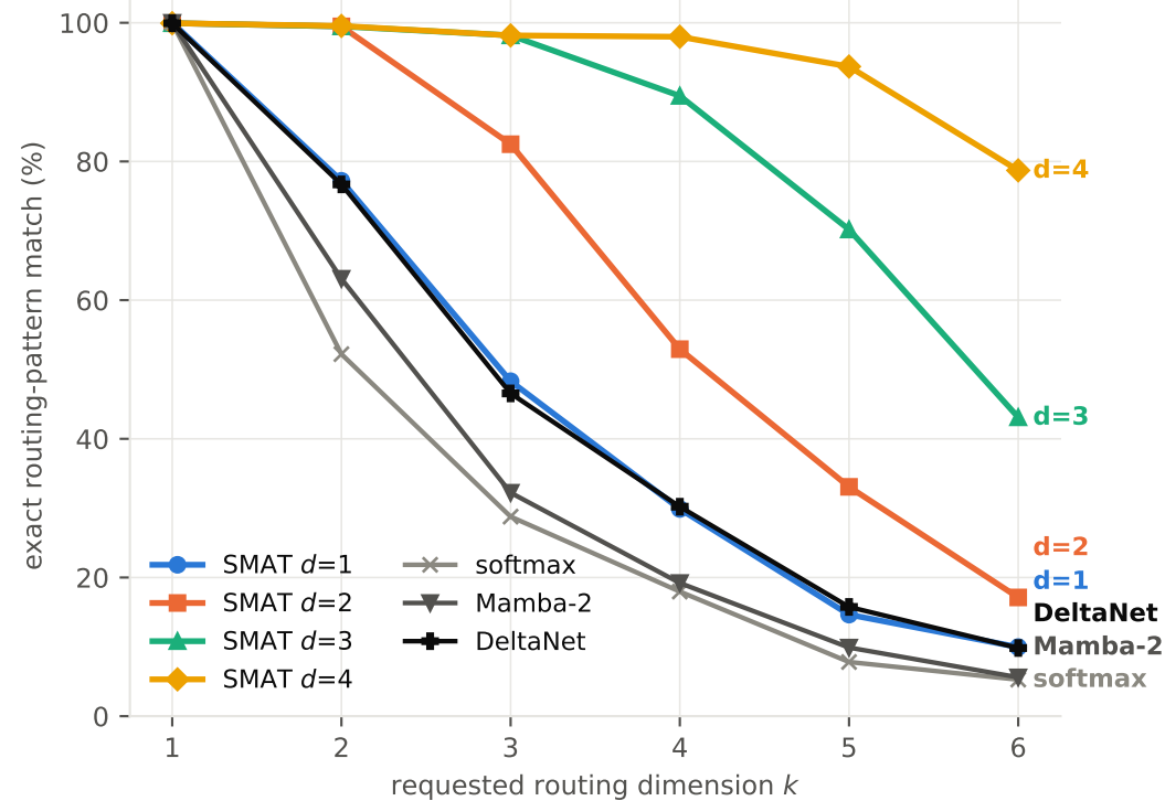
Exact routing-pattern match
