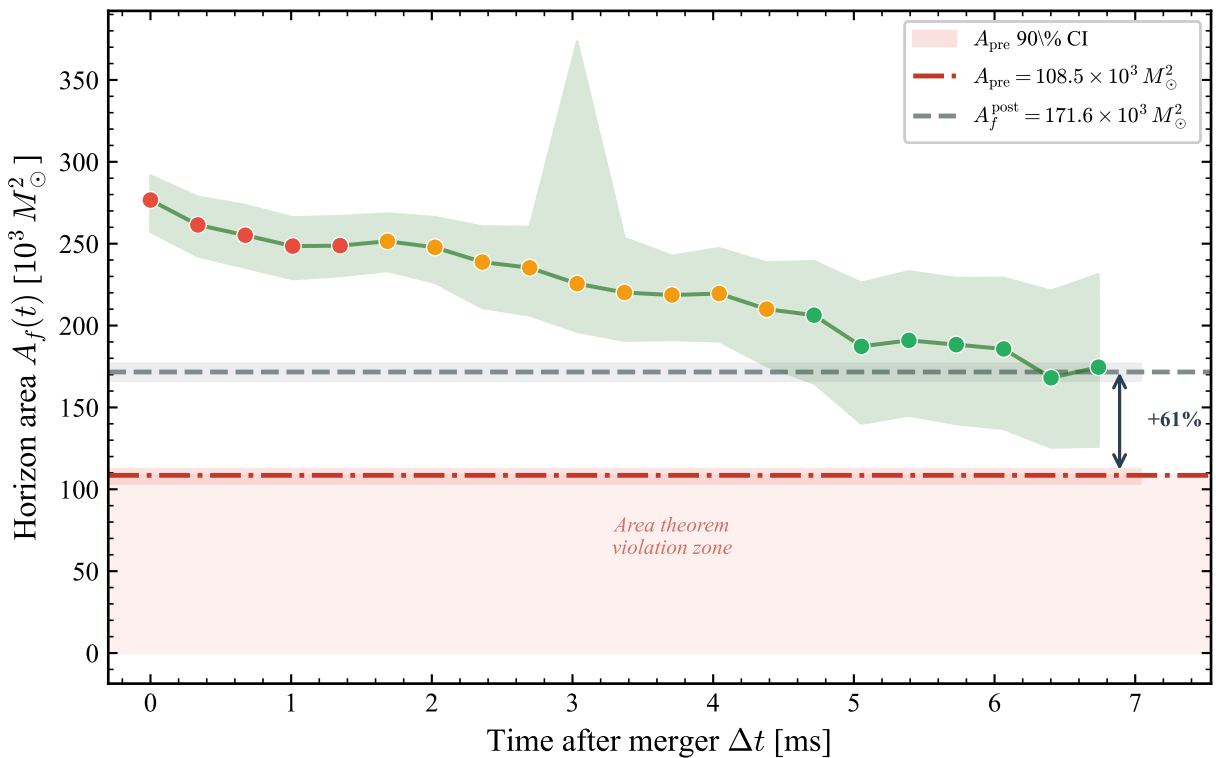
(a) Kerr Horizon Area A_f(t) and Pre-Merger Bound
