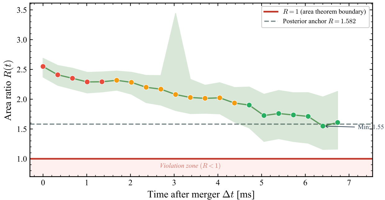
(b) Area Ratio R(t) = A_f(t)/A_{\text{pre}}
