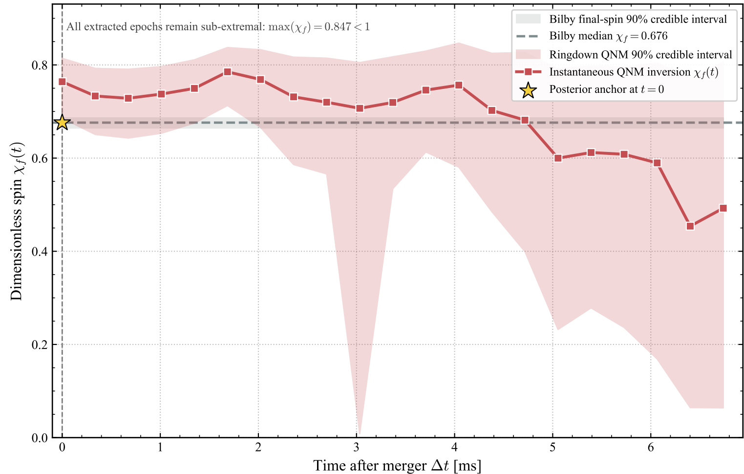
GW250114 Remnant Spin Time Series from Real Ringdown Data
