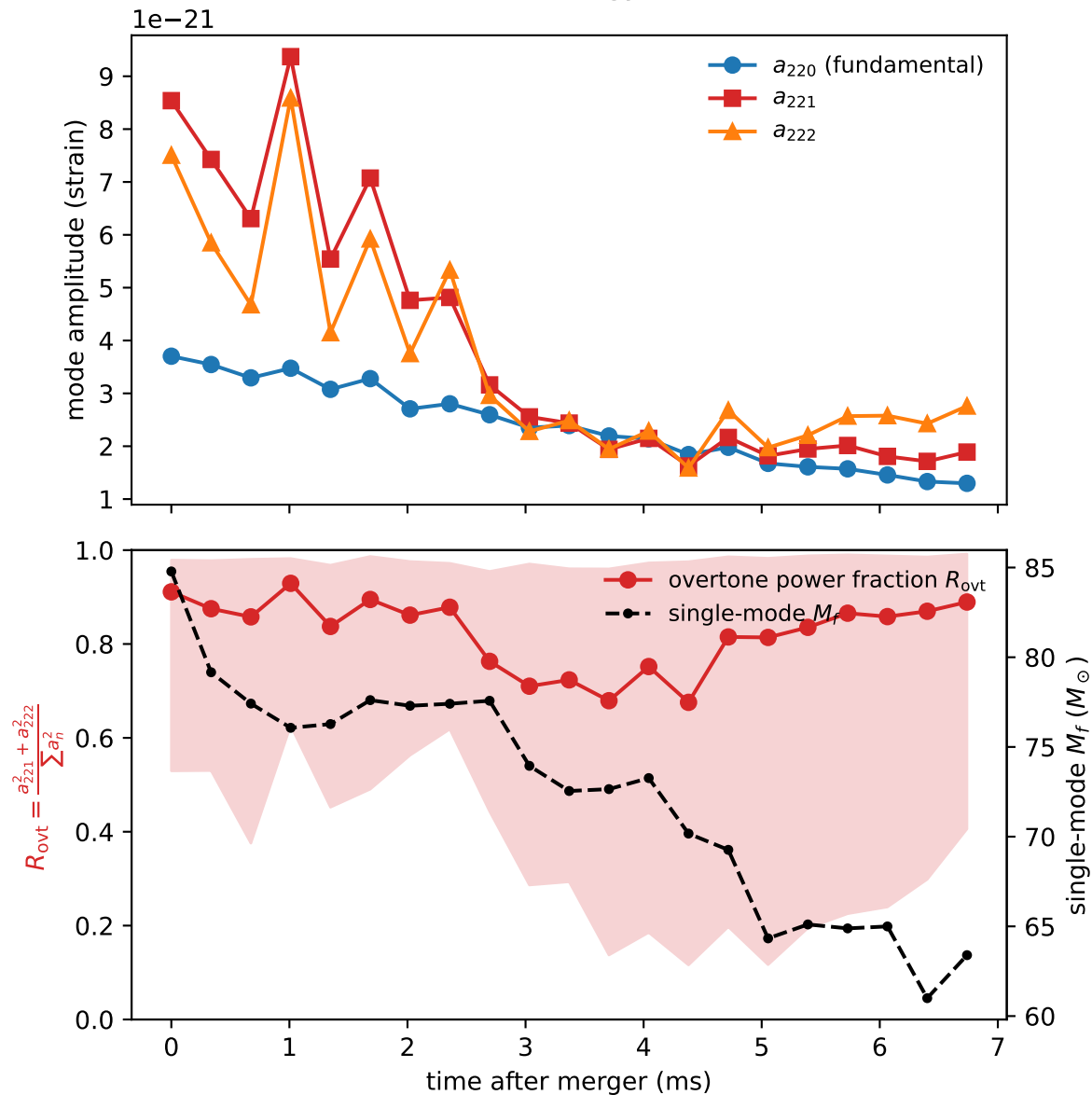
Time-resolved overtone-energy content (GW250114)
