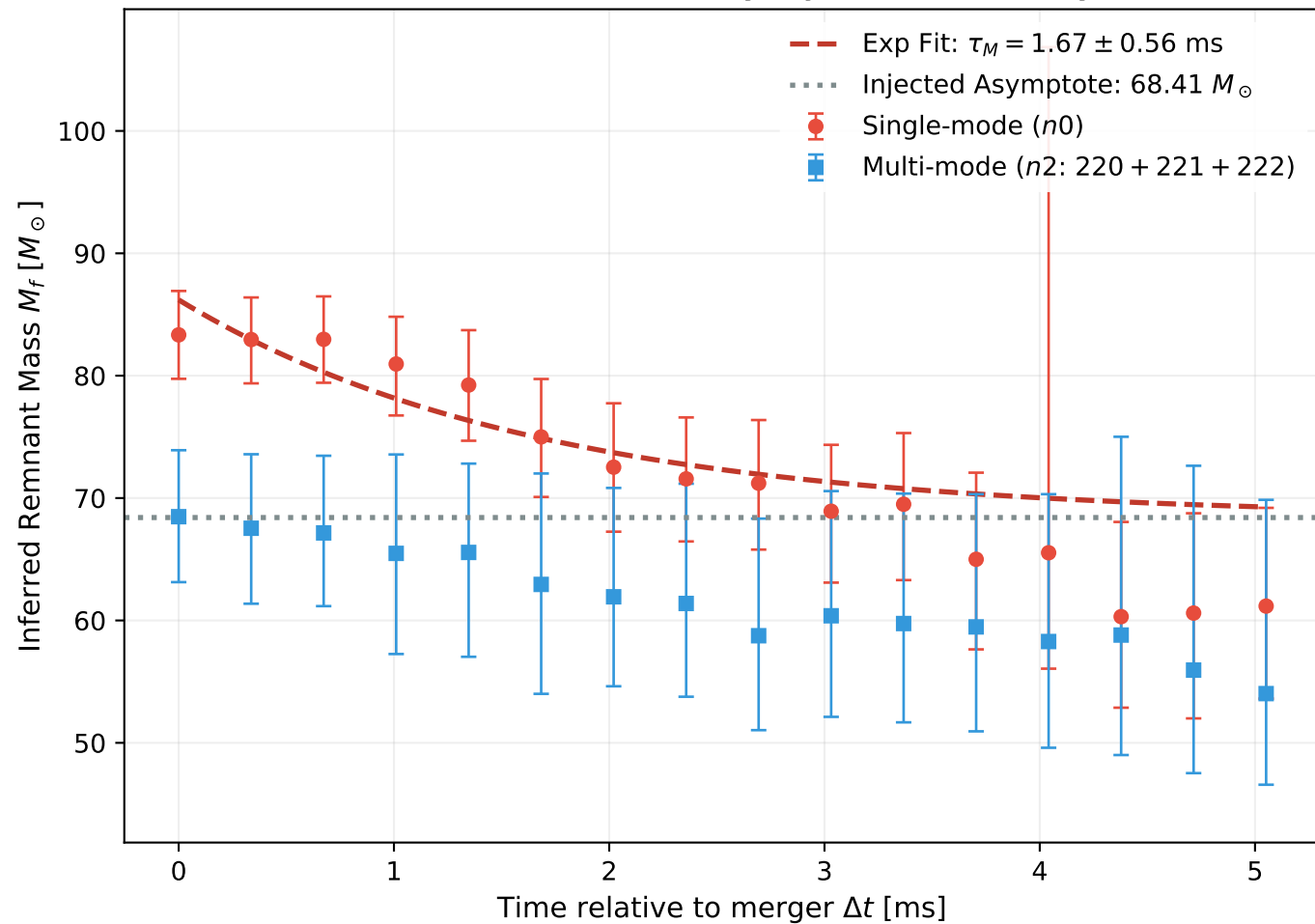
(a) Numerical Relativity Injection Recovery
