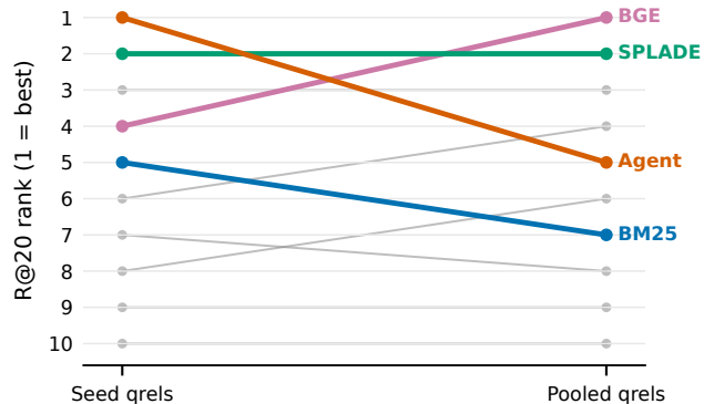
A Ranking changes with qrel construction
