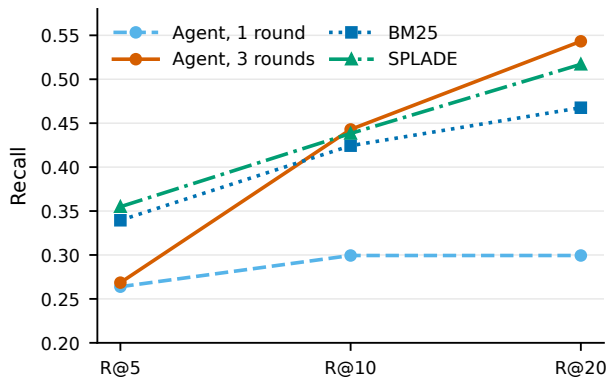
C Iteration increases recall at depth
