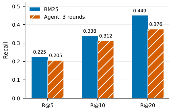
D Cluster-proxy qrels reverse the pairwise result
