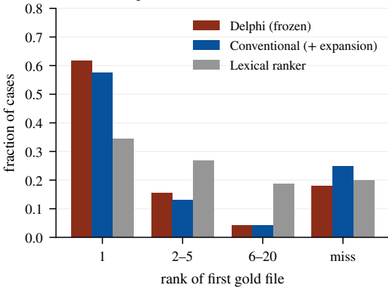
SWE-bench pooled (C0, n=160)
