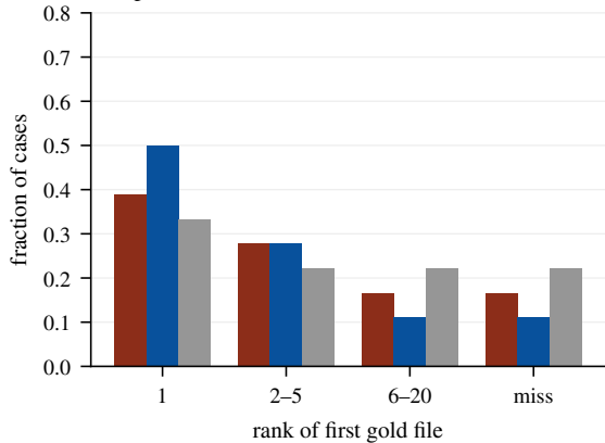
Independent (C0, n=18)
