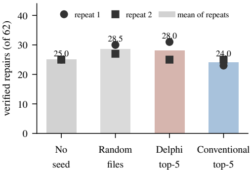
Resolved instances per condition
