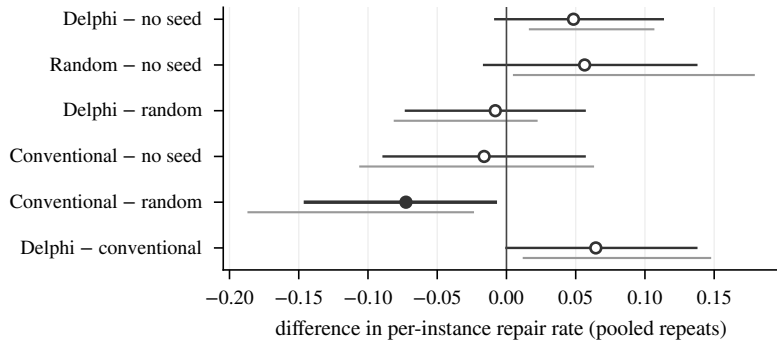
Paired differences; dark: instance-cluster CI, grey: repository-cluster CI
