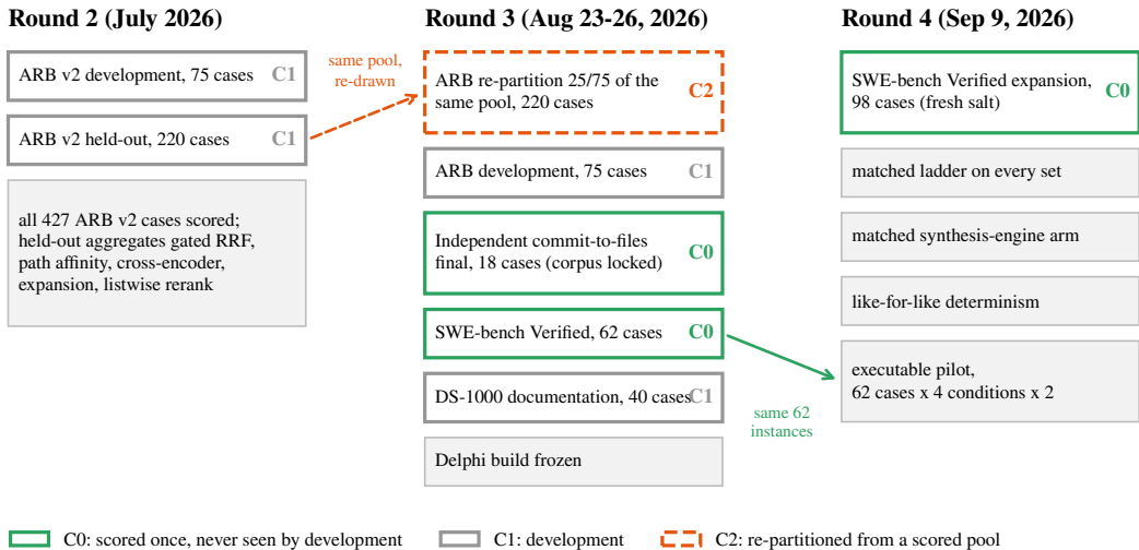
Figure 3: Evaluation rounds, the sets each round scored, and their exposure class. Round 2 scored every case of the ARB v2 pool and used the held-out aggregates to accept components; round 3 re-drew a 220-case partition from that pool (C2) and introduced the first C0 sets; round 4 added the matched ladder, the 98-instance draw, the matched synthesis-engine arm, like-for-like determinism, the executable pilot on the round-3 62-instance set, and, after the confirmatory runs, the factorial, the seed-interface check, and the fresh 60-instance draw for the branch ablation.
