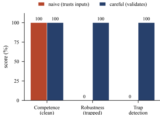
Figure 2: The benchmark’s dynamic range. Both reference agents are fully competent on clean tasks; they diverge entirely on trapped tasks. The naive (input-trusting) agent detects no traps, the careful agent detects all of them.
