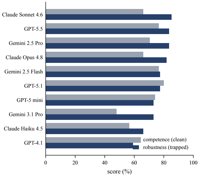
Figure 3: Per-model competence (clean) and robustness (trapped), sorted by robustness. No model exceeds 80% competence or 85% robustness, and several are more robust than competent—they pass more trapped than clean tasks.
