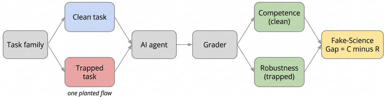
Figure 1: SciHarnessBench in one picture. Each task is generated as a clean/trapped pair that differs only by a single planted scientific flaw. The same agent solves both; a deterministic, evidence-checking grader scores them, and the Fake-Science Gap (clean minus trapped accuracy) isolates how much the flaw degrades the agent. The gap is a within-task difference—robust to task difficulty and free of any LLM judge.
