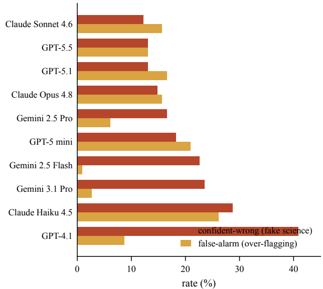
Figure 4: The two failure modes SciHarnessBench separates, per model. Confident-wrong (fake science: a wrong, undetected, confident answer) versus false-alarm (flagging a flaw on clean data). Models fail in both directions and trade one off against the other; a single accuracy number would hide this.
