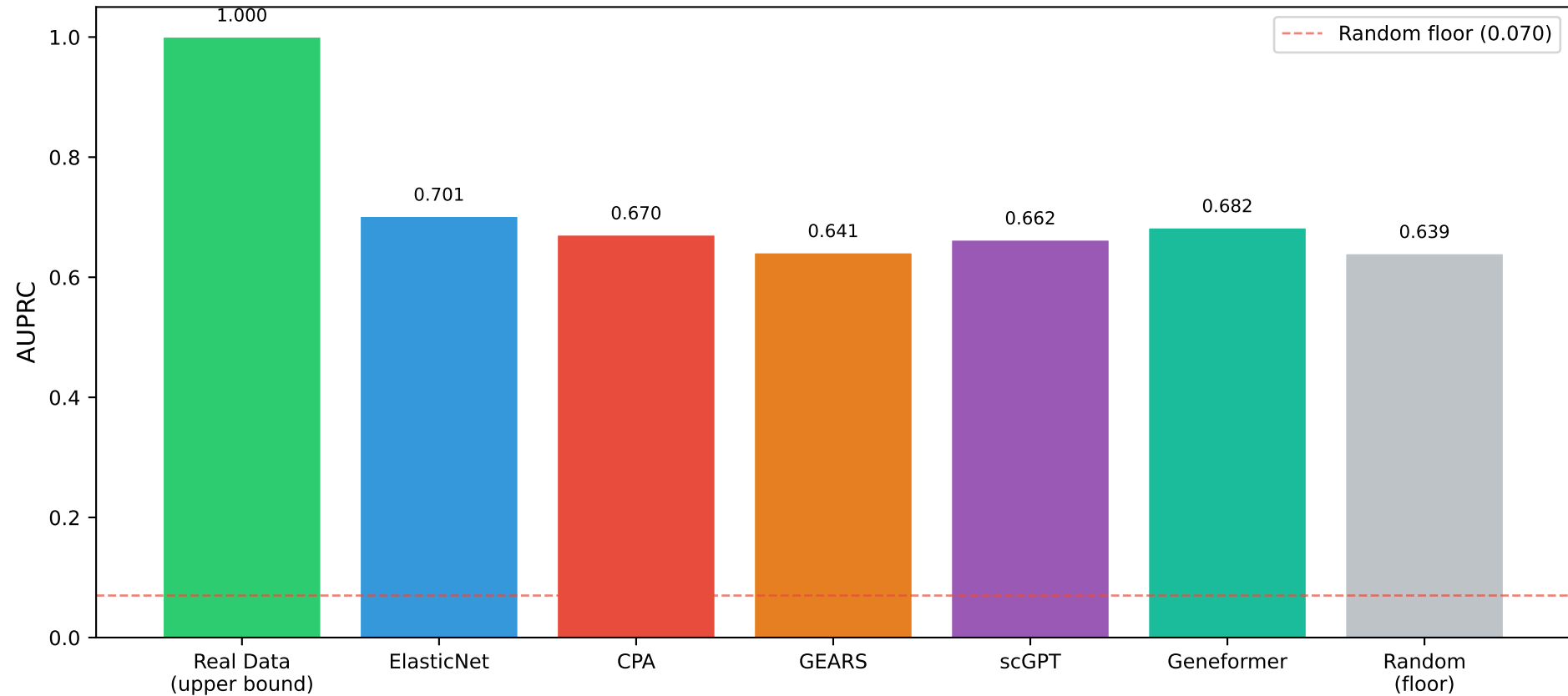
CausalCellBench: Causal Graph Recovery (AUPRC) 100 genes, 10691 control cells
