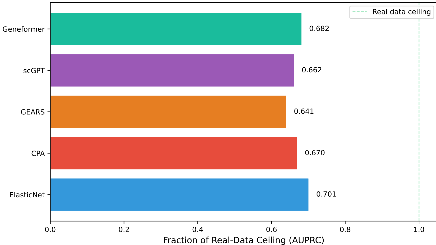
Model Performance as Fraction of Real-Data Ceiling 100 genes
