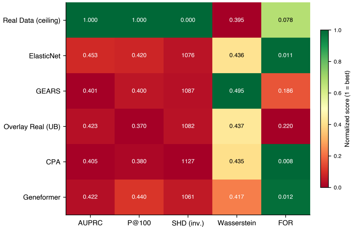
CausalCellBench: Multi-Metric Comparison (200 genes)
