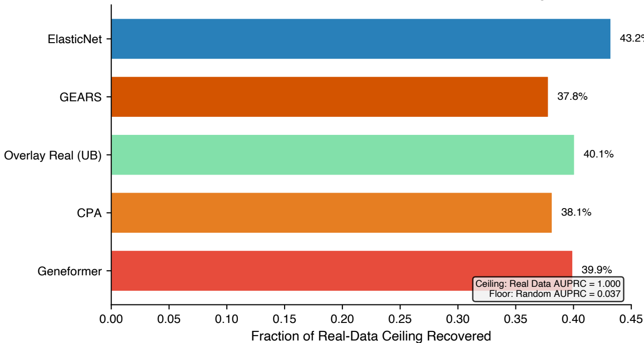
CausalCellBench: Model Performance vs. Real Data (200 genes)
