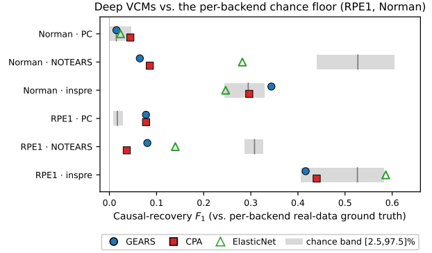
Figure 1. Deep VCM causal-recovery F_1 against the per-backend chance floor on the cross-context (RPE1) and cross-paradigm (Norman) datasets. Each row is one (dataset, backend) cell; the grey band is the permutation-null [2.5, 97.5] chance interval (vertical tick at the null mean; K=30 permutations, 24 for PC on Norman). Markers are GEARS (circle), CPA (square), and the ElasticNet comparator (open triangle). Deep markers inside the band are at chance, left of it are below chance, right of it are above chance. Both deep models land inside or below the band in four of six cells; two cells hold an above-band deep point—PC on RPE1 (both models, observational co-expression at F_1 = 0.078 ) and GEARS under inspre on Norman (a single-seed margin above the band edge)—neither exceeding the linear comparator. ElasticNet matches or exceeds both deep models in every cell where it is defined. n_{gt} ground-truth edges per cell range from 67 to 1,327.
