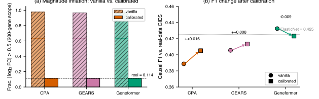
Figure 6. Effect-size calibration corrects magnitude distribution exactly but only partially recovers causal F_1 . (a) Fraction of |\log_2 \text{FC}| > 0.5 before (hatched) and after (solid) quantile-matching calibration for each deep model on the K562 200-gene scope; the dashed horizontal line marks the real-data 200-gene reference. (b) Causal F_1 against the real-data GIES ground truth before (circles) and after (squares) calibration on the identical pipeline (seed 42, partition size 20); arrows connect paired vanilla and calibrated values. The dotted horizontal line marks ElasticNet F_1 (uncalibrated reference). n = 1 seed \times 200 perturbations \times 200 genes.
