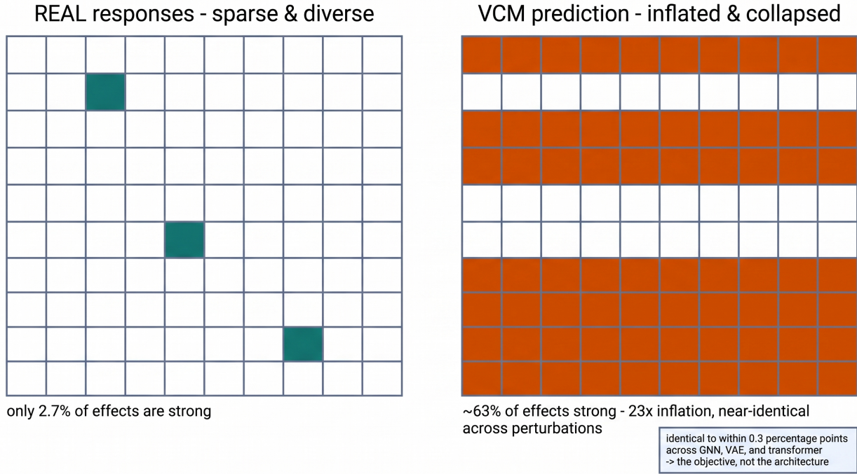
Figure 8. Mode collapse as an objective-level, architecture-independent failure (schematic companion to Figure 4 and Table 12). Real perturbation responses are sparse—only 2.7% of (perturbation, gene) effects are strong (left, teal). Deep VCM predictions inflate this to \approx 63\% (right, vermillion), a \sim 23 -fold inflation that is nearly identical across perturbations and identical to within 0.3 percentage points across GEARS (GNN), CPA (VAE), and Geneformer (transformer)—indicating the failure is driven by the shared training objective rather than architecture, consistent with the ablation above.
