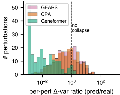
(a) Per-pert variance compression
