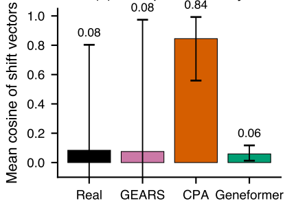
(b) Inter-pert similarity
