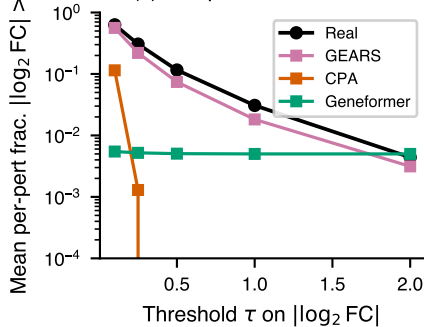
(c) Per-pert inflation curve
