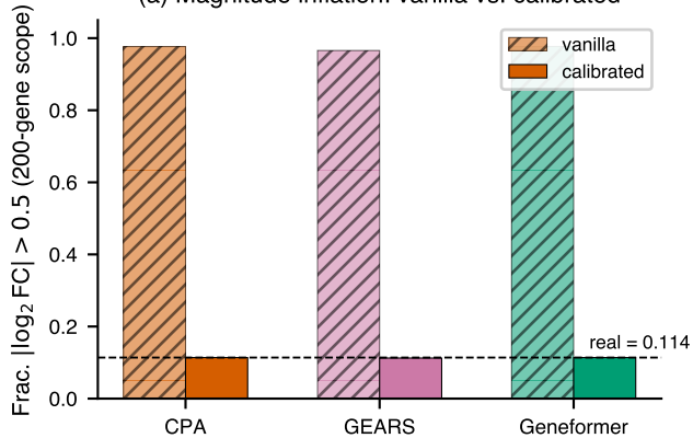
(a) Magnitude inflation: vanilla vs. calibrated
