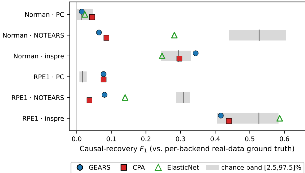
Deep VCMs vs. the per-backend chance floor (RPE1, Norman)
