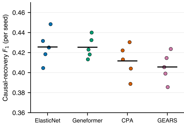
Per-seed F_1 across 5 seeds ( N = 200 K562)
