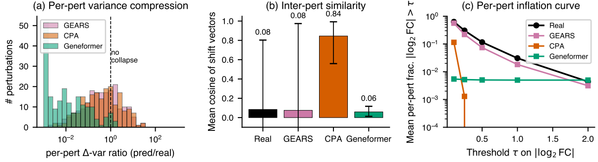
Figure 3. Mode-collapse vs. inflation reconciliation diagnostic on K562 ( N=200 , 193 perturbations). (a) Per-perturbation \Delta -variance ratios (dashed line: ratio = 1); all deep models compress, Geneformer by \sim two orders of magnitude. (b) Inter-perturbation cosine similarity (whiskers p_{10} – p_{90} ); CPA produces nearly the same response across perturbations (0.84 vs. 0.08 real). (c) Mean per-perturbation fraction |\log_2 \text{FC}| > \tau vs. threshold \tau ; deep models track real or fall below per-perturbation yet exceed real at the full-transcriptome pool. Full panel descriptions in §C.1.
