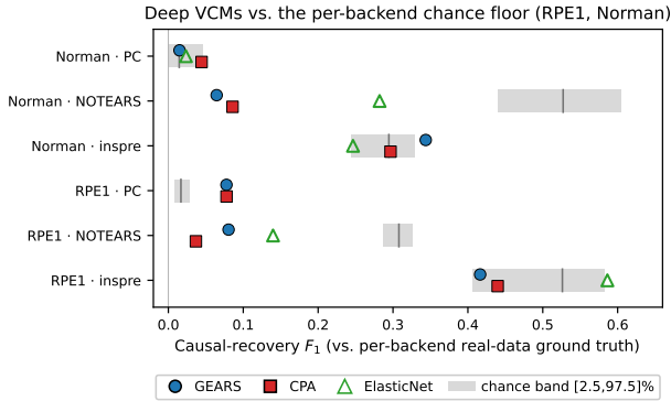
Figure 1. Deep VCM causal-recovery F_1 against the per-backend chance floor on RPE1 and Norman. Each row is one (dataset, backend) cell; the grey band is the permutation-null [2.5, 97.5] chance interval ( K=30 permutations, 24 for PC on Norman). Markers are GEARs (circle), CPA (square), and the ElasticNet comparator (open triangle). Both deep models land inside or below the band in four of six cells; the two above-band points (PC on RPE1 at F_1 = 0.078 ; GEARs under inspre on Norman, a single-seed margin) neither exceed the linear comparator nor reach substitutable quality. n_{gt} ground-truth edges per cell range from 67 to 1,327.
