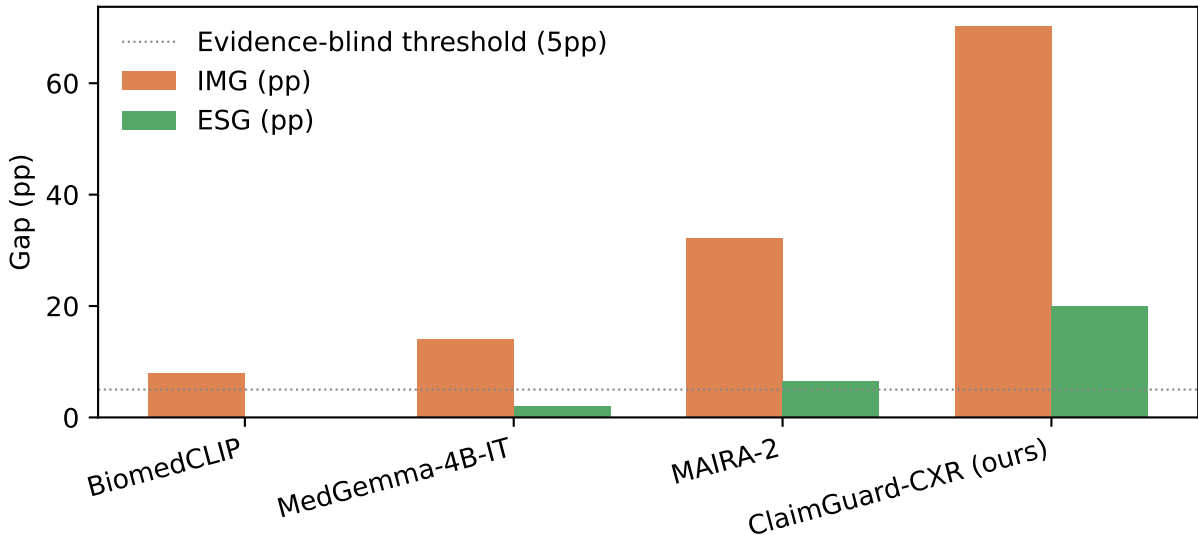
Baseline landscape on real-RRG claims
