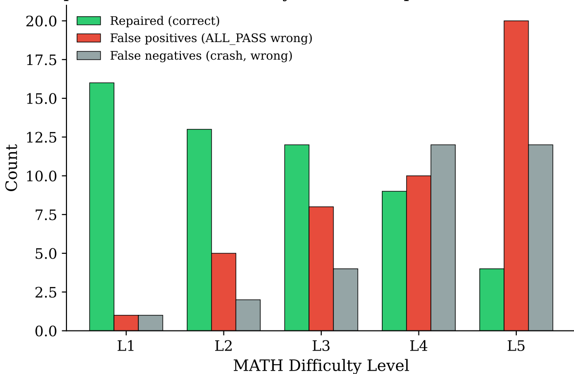
Verification Outcome Distribution by Difficulty Repairs concentrated at easy levels; false positives at hard levels
